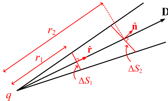
Figure 9: When a sliver of angular sector is taken, same amount of electric flux from a point charge passes through two incremental surfaces \Delta S_1 and \Delta S_2 .
