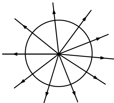
Figure 7: Electric flux from a point charge satisfies Gauss's law.
