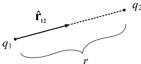
Figure 3: The force between two charges q_1 and q_2 . The force is repulsive if the two charges have the same sign.
