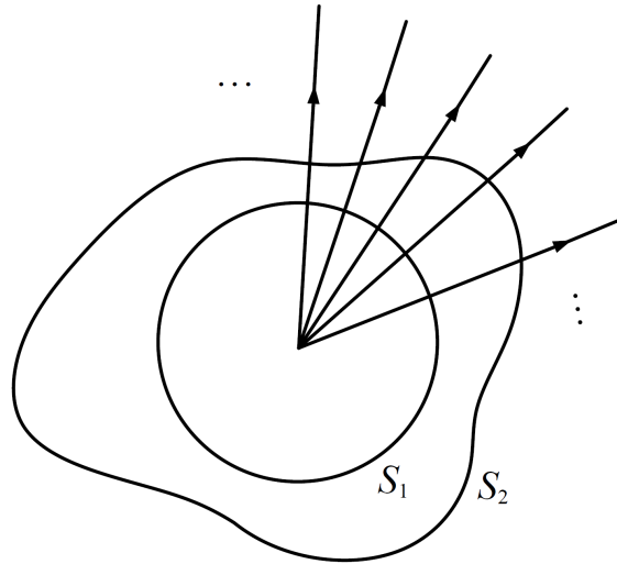
Figure 8: Same amount of electric flux from a point charge passes through two surfaces S_1 and S_2 .
