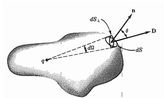
Figure 6: Electric flux (Courtesy of Ramo, Whinnery, and Van Duzer)
