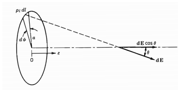
Figure 5: Electric field of a ring of charge (Courtesy of Ramo, Whinnery, and Van Duzer).
